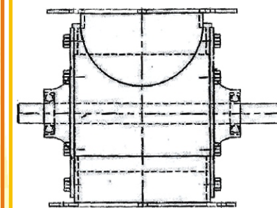
Ash Feeder
