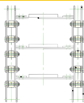
Drag Chain
